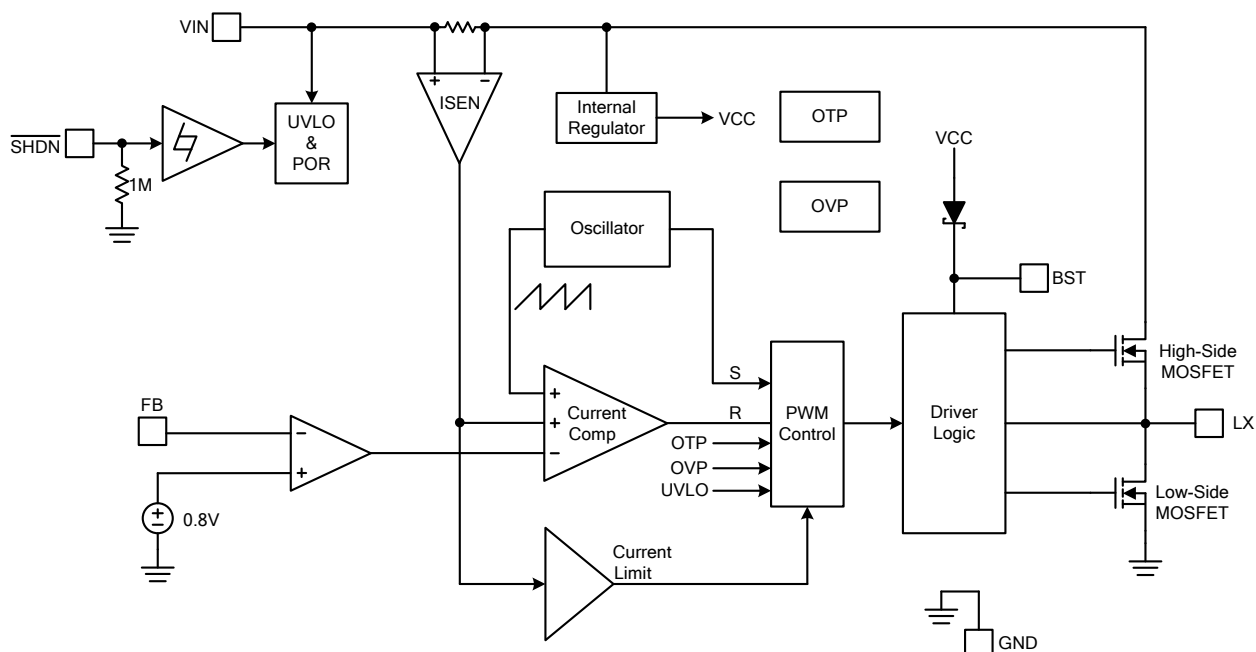
Figure 4. Block Diagram of FR9801
