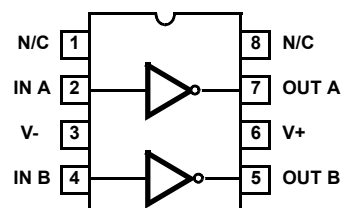
ICL7667 (8 LD PDIP, SOIC) TOP VIEW
