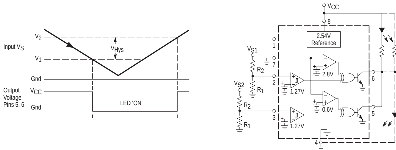
Figure 15. Dual Positive Overvoltage Detector
