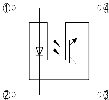
Internal connection diagram (Common to 4 models )
