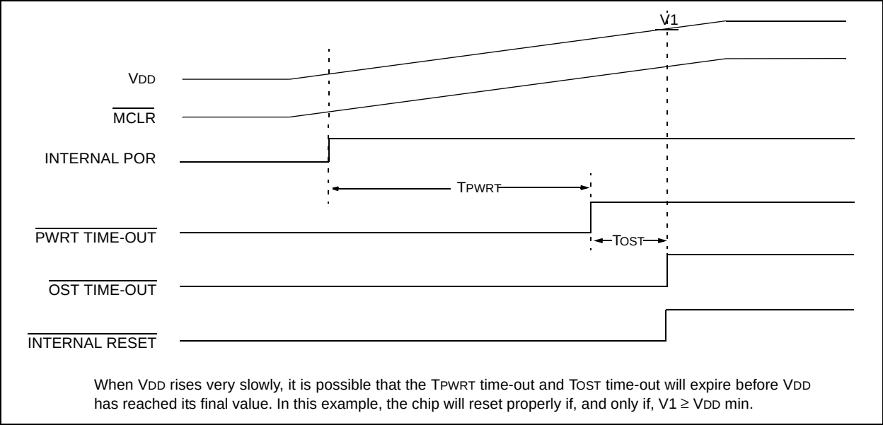
FIGURE 6-9: TIME-OUT SEQUENCE ON POWER-UP (MCLR TIED TO VDD): SLOW VDD RISE TIME
