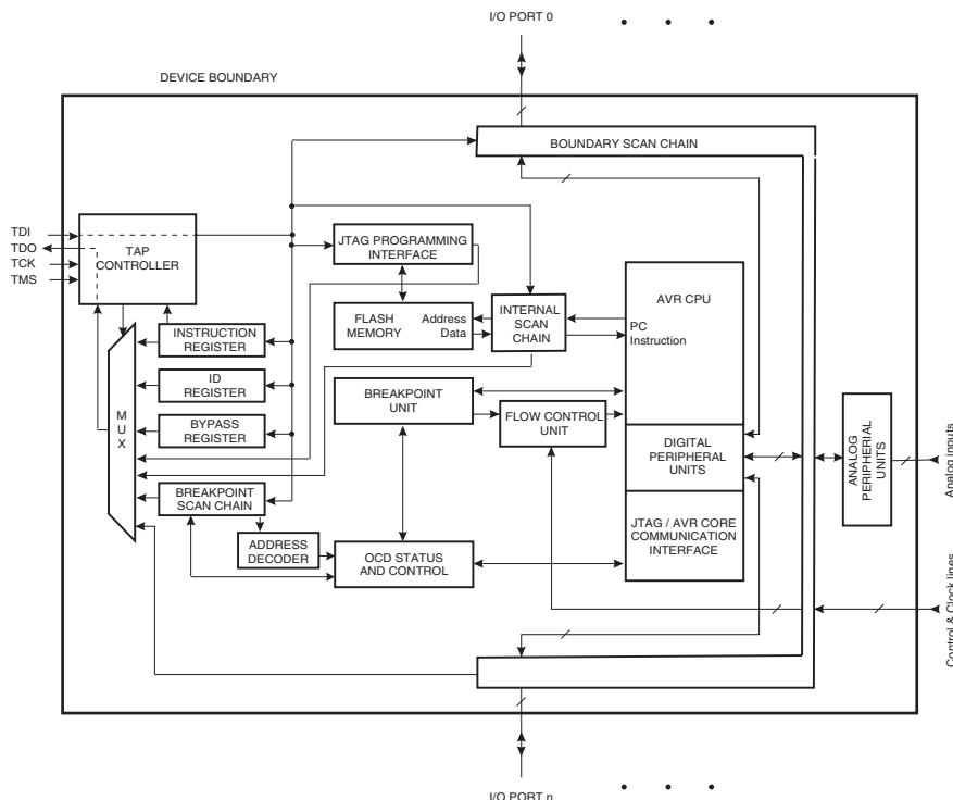
Figure 24-1. Block Diagram
