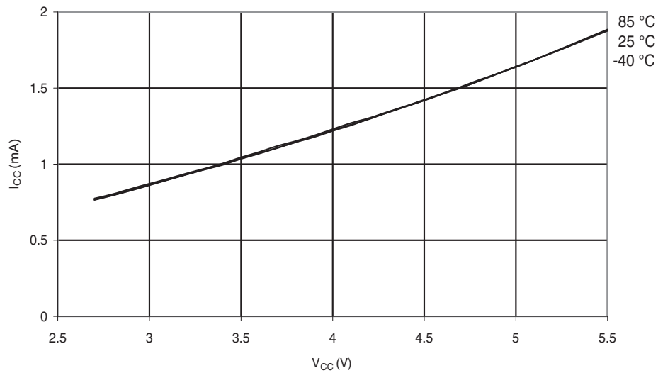
Figure 28-3. Active Supply Current vs. V_{CC} (Internal RC Oscillator, 1MHz)
