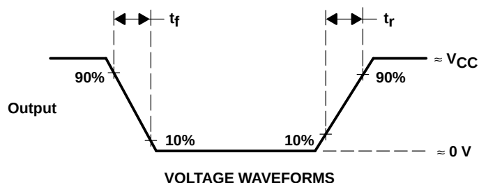
Figure 2. Switching Times
