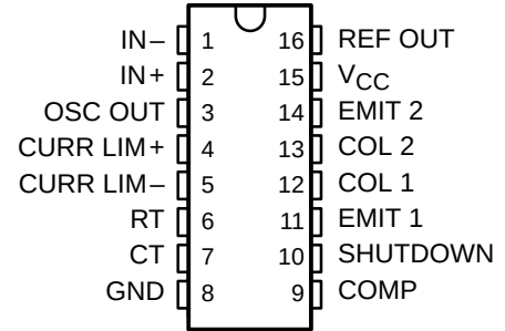
D OR N PACKAGE (TOP VIEW)
