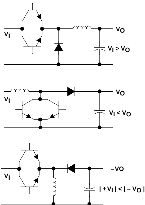
Figure 10. Single-Ended Inductor Circuit
