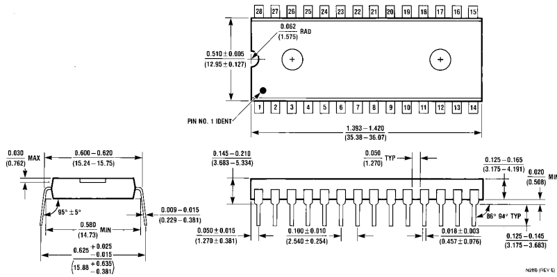
Dual-In-Line Package (N) Order Number NMC27C64N NS Package Number N28B
