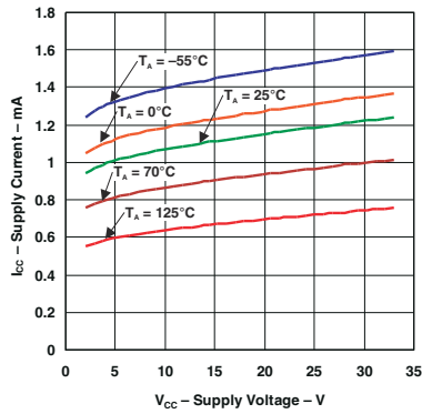
Figure 6-1. Supply Current vs Supply Voltage
