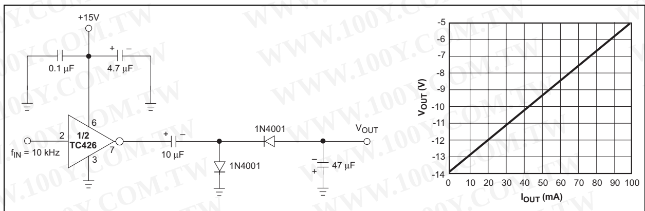
FIGURE 3-4: Voltage Inverter
