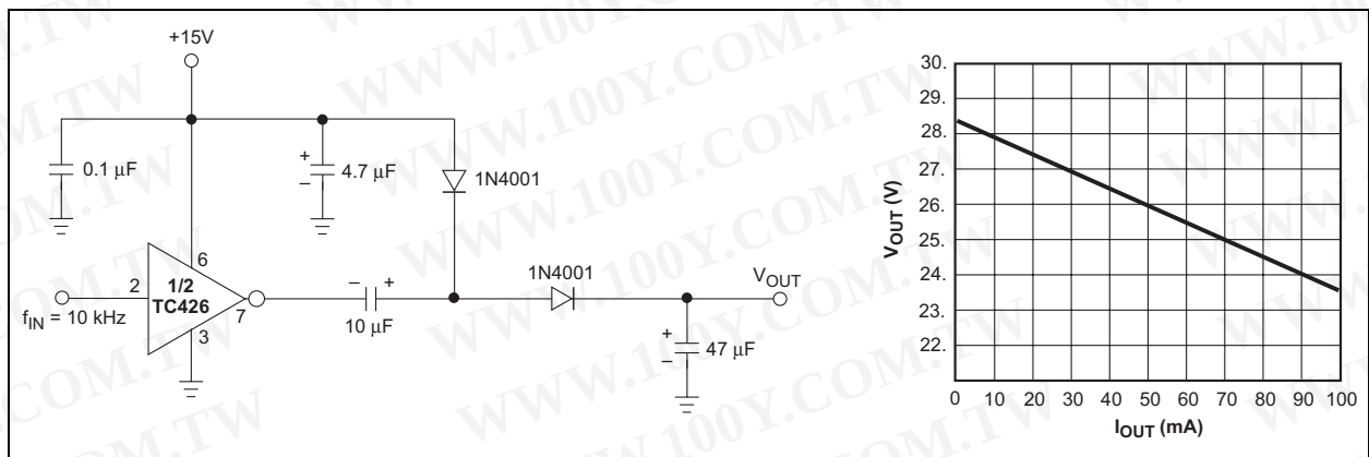
FIGURE 3-3: Voltage Doubler
