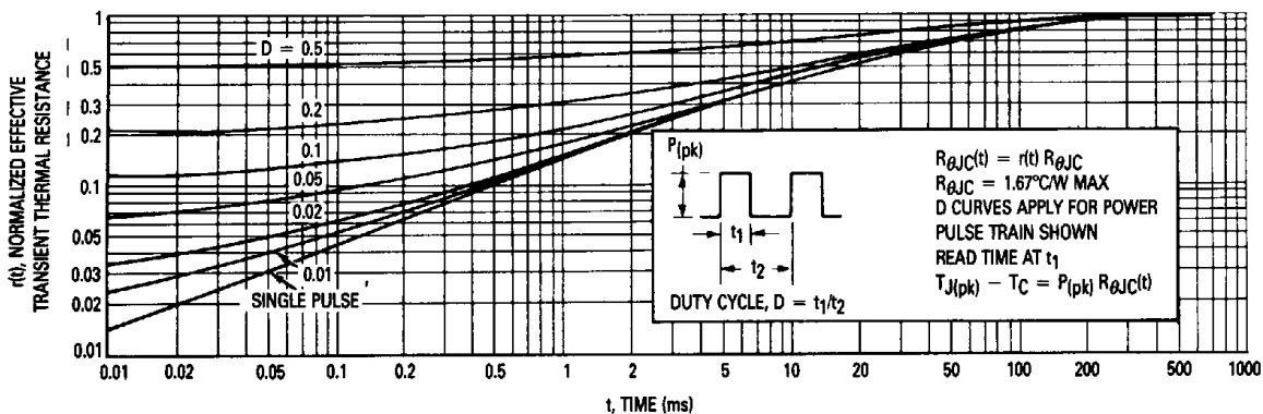
Figure 10. Thermal Response
