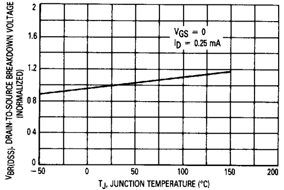
Figure 4. Normalized Breakdown Voltage versus Temperature
