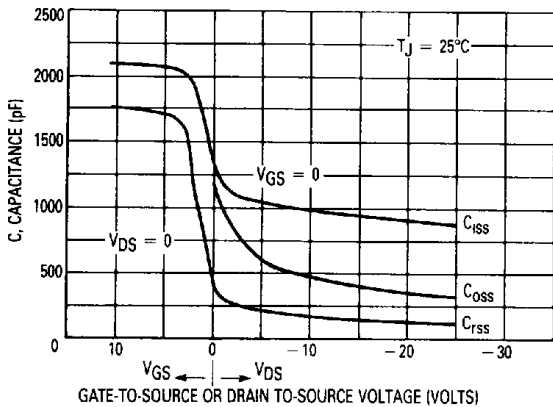
Figure 11. Capacitance Variation
