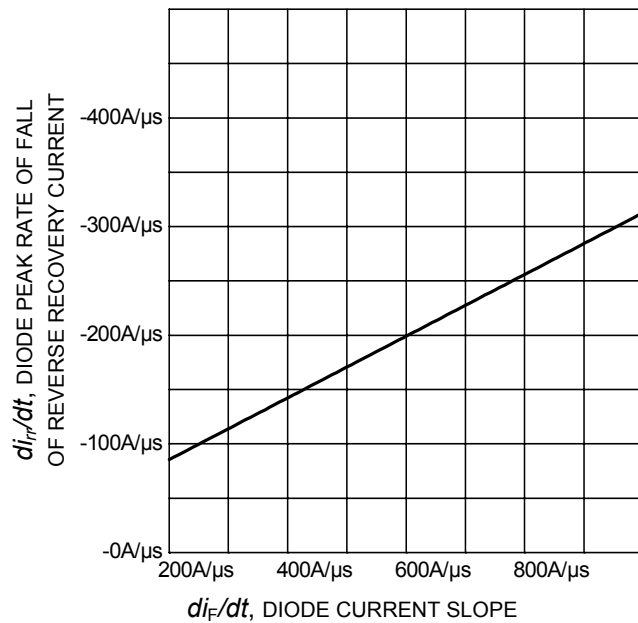
di_F/dt , DIODE CURRENT SLOPE Figure 24. Typical diode peak rate of fall of reverse recovery current as a function of diode current slope ( V_R=400V , T_J=150^\circ C , Dynamic test circuit in Figure E)
