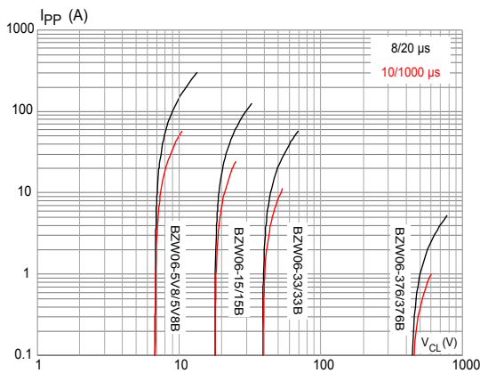
Figure 5. Maximum peak pulse current versus clamping voltage
