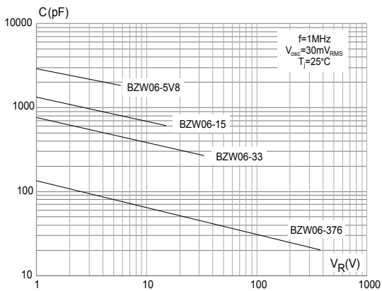
Figure 7. Junction capacitance versus reverse applied voltage (unidirectional type)
