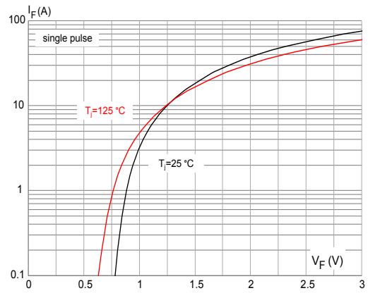
Figure 10. Peak forward voltage drop versus peak forward current
