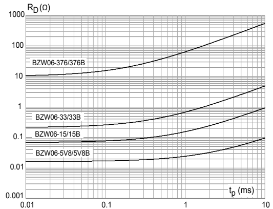
Figure 6. Dynamic resistance versus pulse duration
