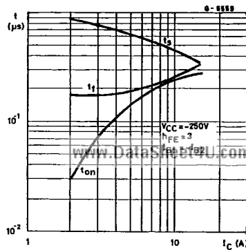
Saturated Switching-times Resistive Load.
